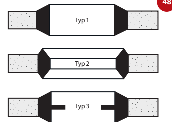
BS - Bonded seals (Gummi-Stahl Verbund)
